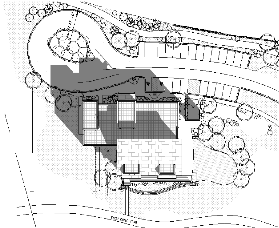
① SHADOW PLAN - Dec. 21 - 9am 1" = 40'-0"
